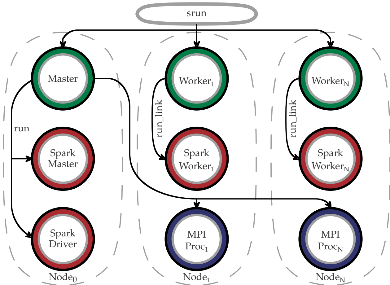
Figure 3.2 Colored processes implicitly communicate during startup. Arrows show connections between Slurm and the supervisor, and between the supervisor and its child processes.
