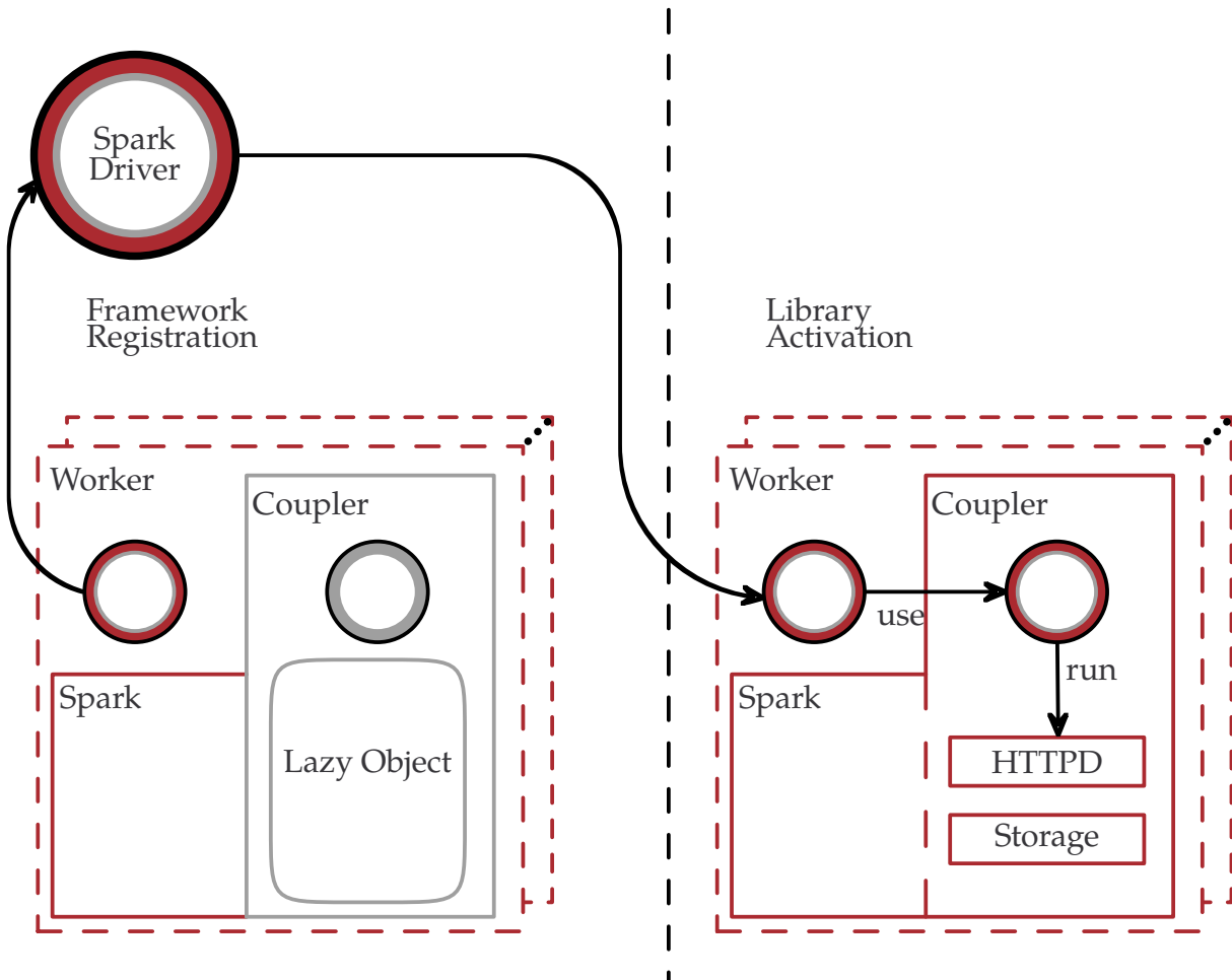
Figure 3.5 Because of Spark’s implicit parallelism, the code for the coupler depicted here is part of every Spark process. As shown on the left, the actual object does not exist at first. When instantiated, the coupler contains the implementation of the transport described in the preceding sections.
