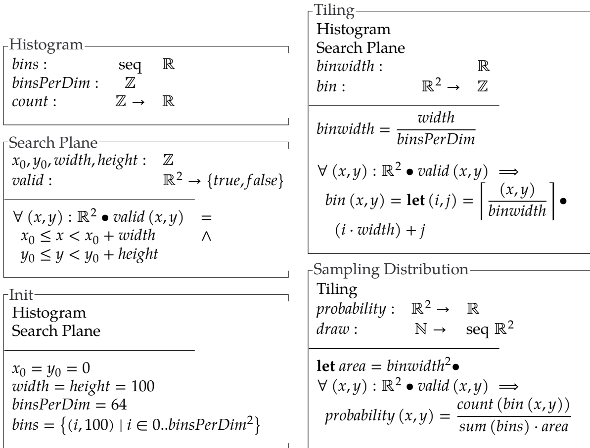
Figure 4.6 Both halves of the demo use the same model for histograms discretizing a search space. The monte-carlo search process initializes its histogram to a uniform positive value and uses it to drive its sampling distribution. The given parameter values correspond to the output graphs later in this section.
