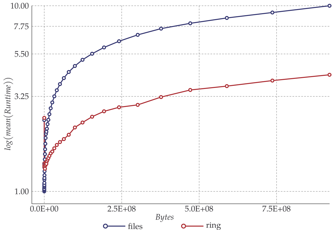
Figure 4.3 Comparing Filesystem (files) and Ring-Buffer (ring) Transports: Runtime with Increasing Size
