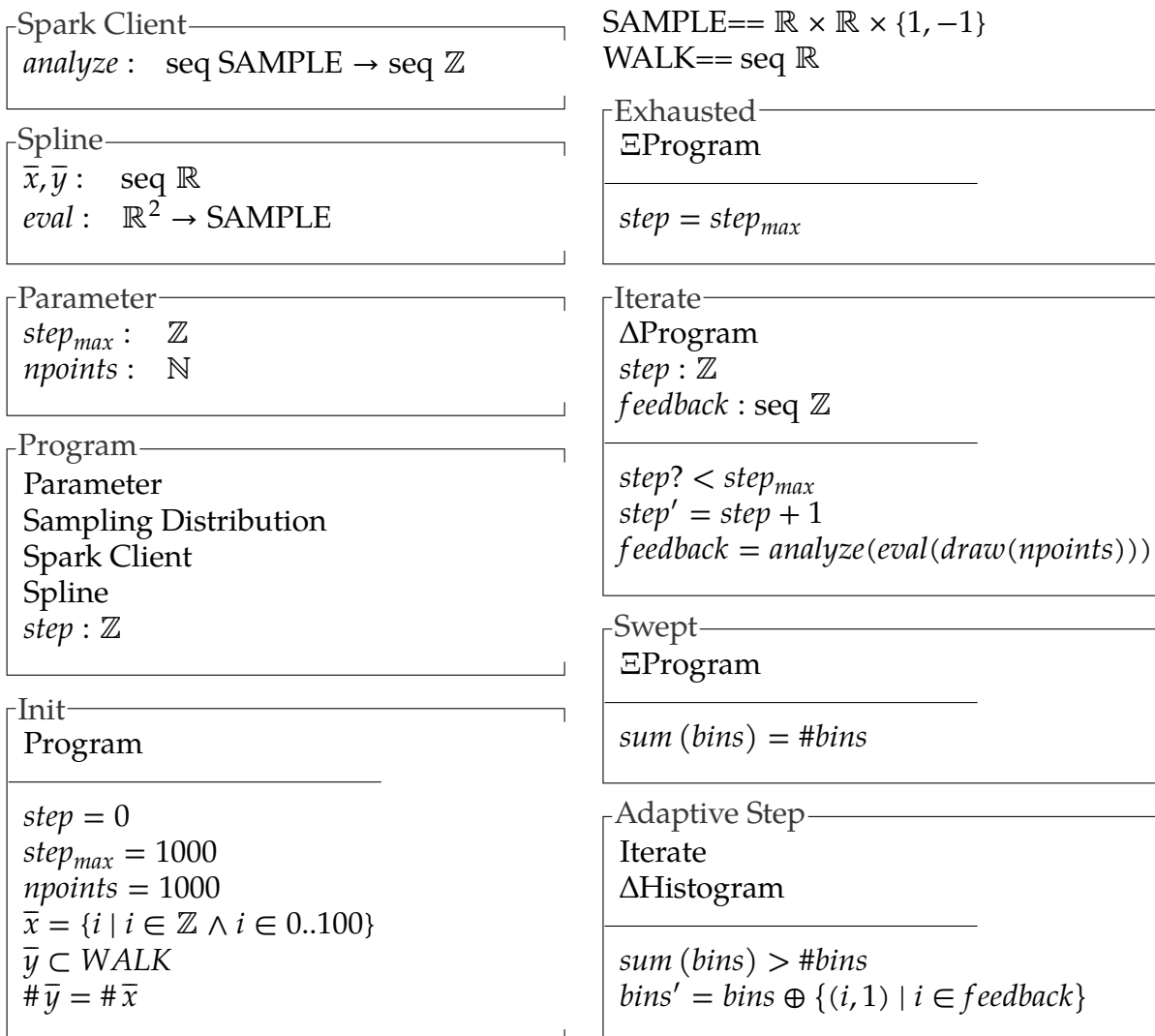
Figure 4.7 Spark feedback can be used to update the probability distribution. While a more complex model is easily enabled by letting Spark choose new values for each bin, this simple version merely sets bin values to one when Spark returns their indices.
