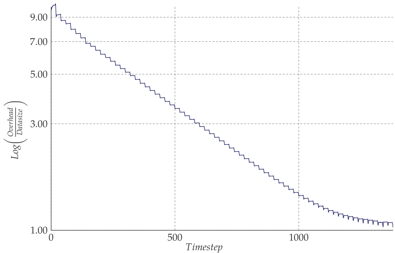
Figure 4.2 Ratio of Overhead to Data Size for Increasingly Large Data Steps
