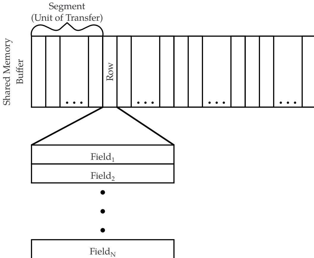
Figure 3.3 The “Ring” in “Ring Buffer” contains indexed segments comprised of rows. In a fully-threaded implementation, segments could be randomly accessible and lockable, but our single-producer-consumer paired version uses semaphores and a single modular counter instead. All segments are transferred only when full, except for the very last, which is allowed to be partially empty.
