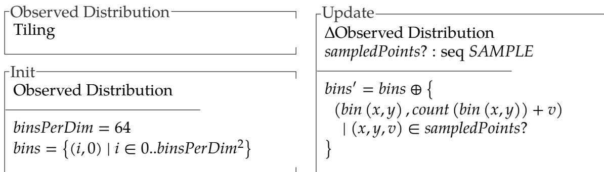
Figure 4.8 Updating Observed Distribution
