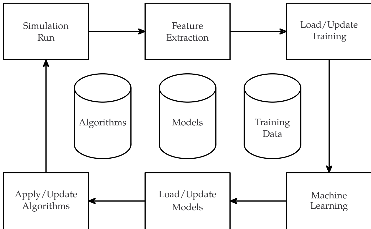
Figure 1.1 Traditional Coupled Workflows
