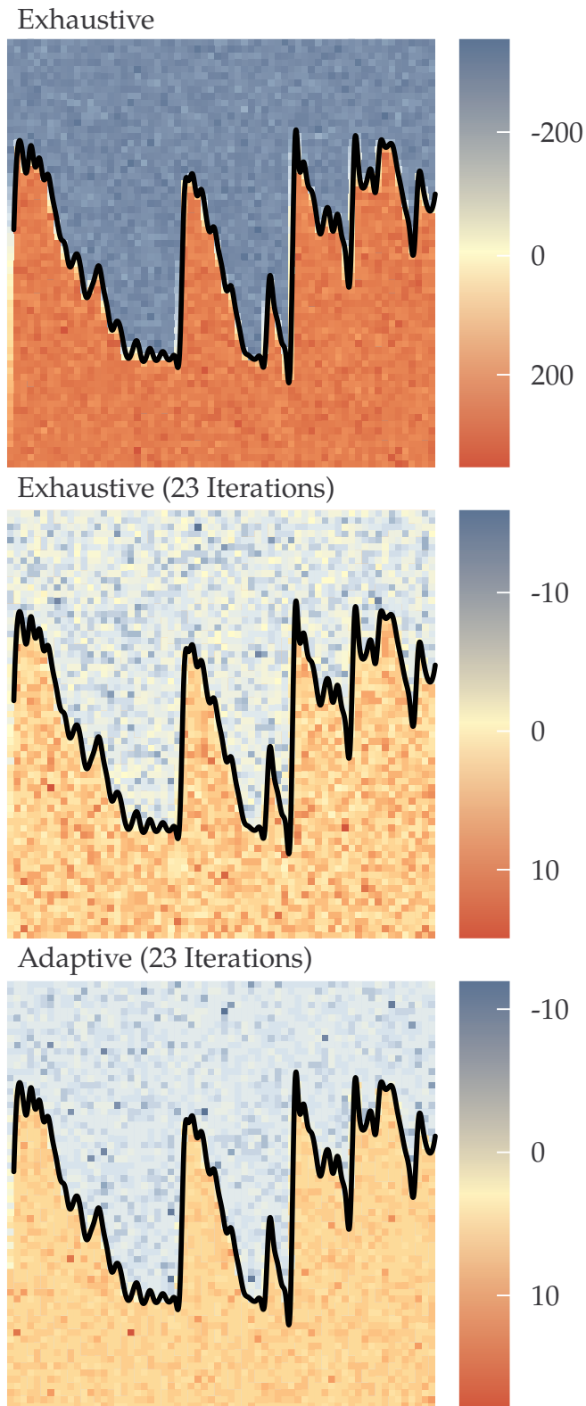
Figure 4.10 Adaptive Monte Carlo quickly terminates while maintaining good space coverage. Non-adaptive programs of the same length produce noisy, low-quality output.
