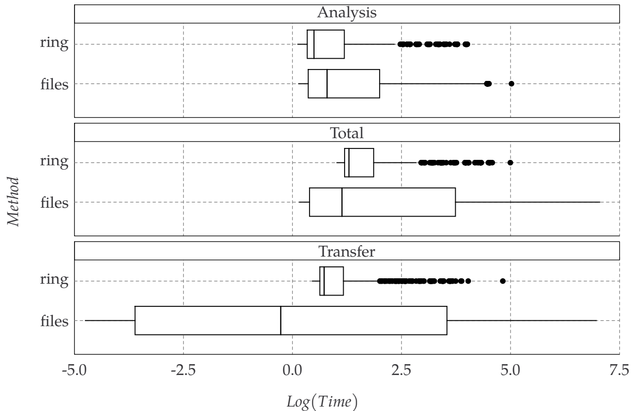
Figure 4.4 Comparing Filesystem (files) and Ring-Buffer (ring) Transports: Time Distribution
